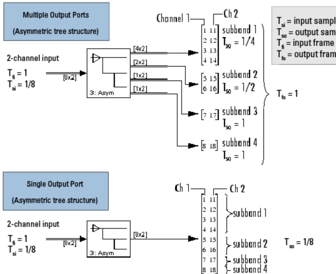
Outputs of a 3-Level Asymmetric Dyadic Analysis Filter Bank
